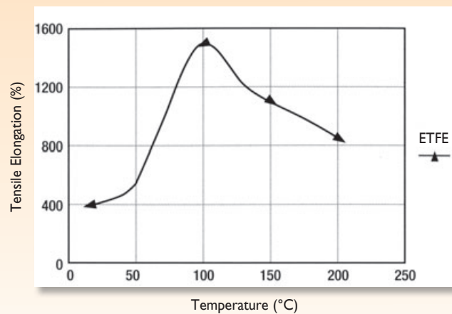
Effect of Temperature on Tensile Elongation
