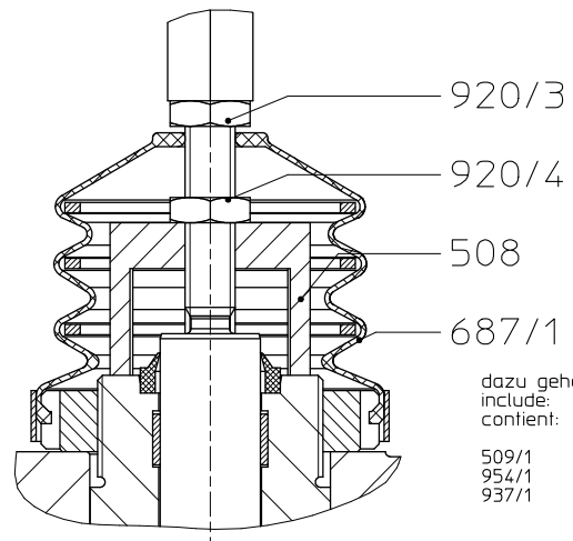
Option travel stop
