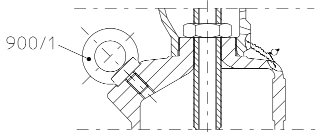
View W
