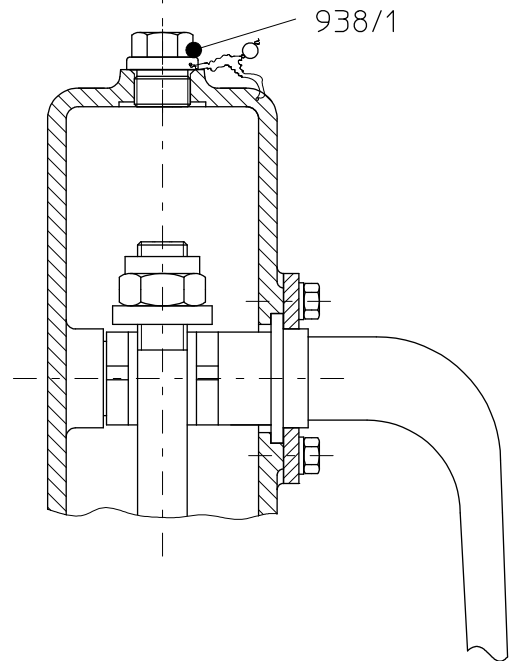
View W
