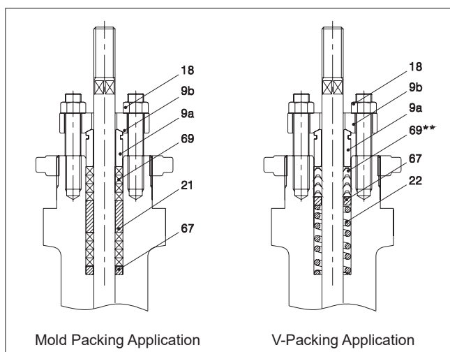
Fig. 6 Gland packing
