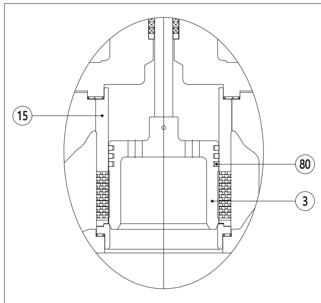
Fig. 9 High temp balanced trim
