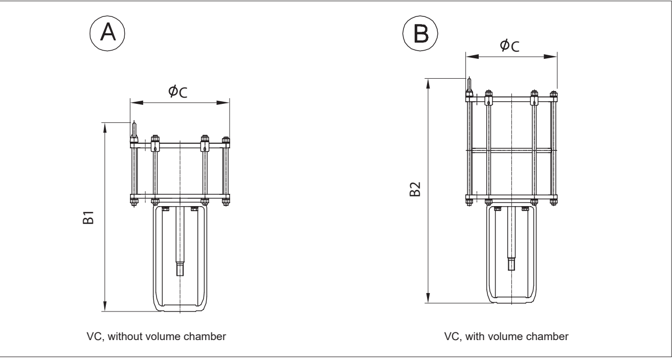
VC actuator without handwheel
