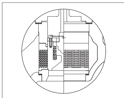
Omega quick change, Pilot balanced trim
