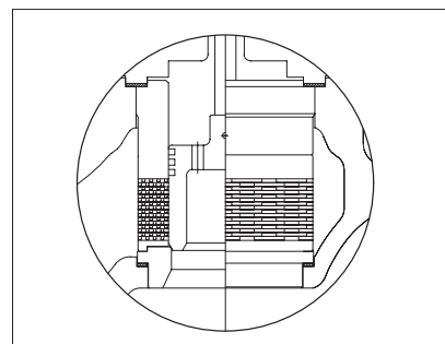
Omega quick change, High temperature balanced trim
